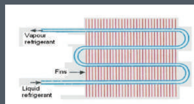
Air cooled Condensers made of Copper tubes with Aluminium fins offering highest rate of heat transfer
